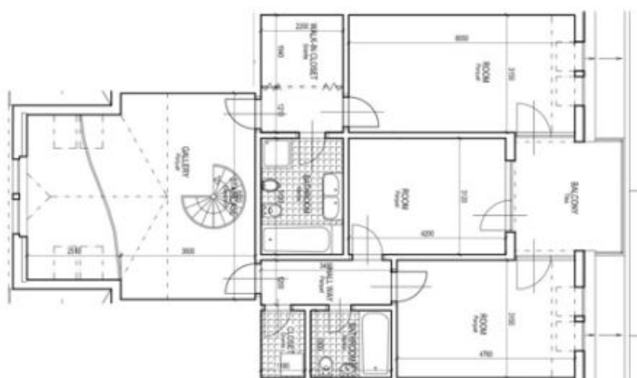
SIXTH FLOOR
