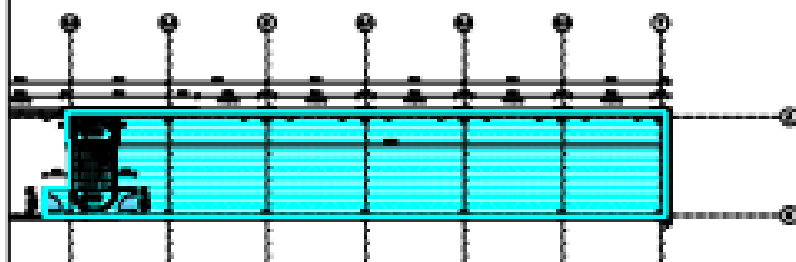
PŮDORYS 2NP / 2nd floor plan
